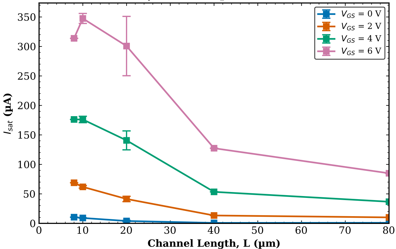
TFT1 Combined (Tr. 1 & 2) I_{sat} vs L | W = 500 \mu\text{m} (mean \pm std)
